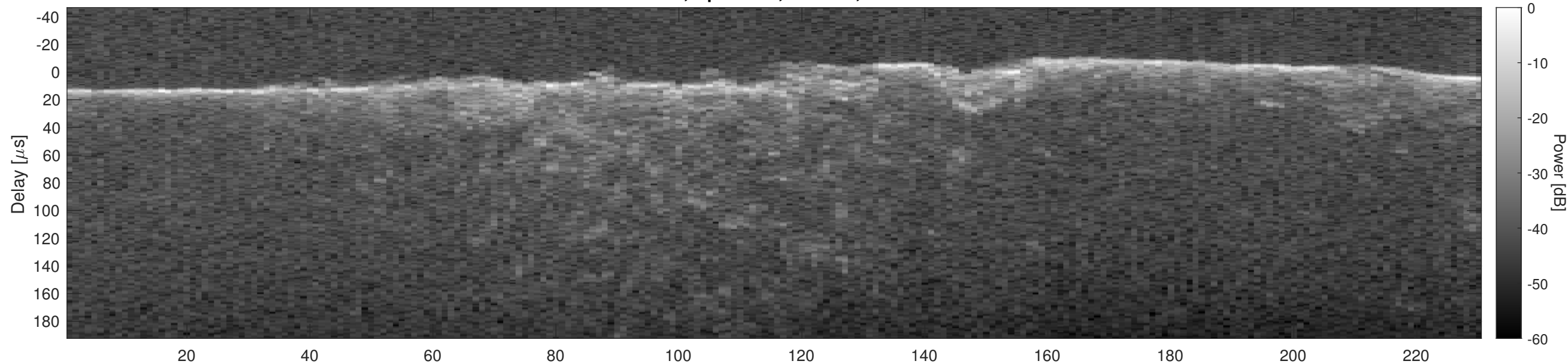
Orbit 9269, Optimized, Window, Channel 2
