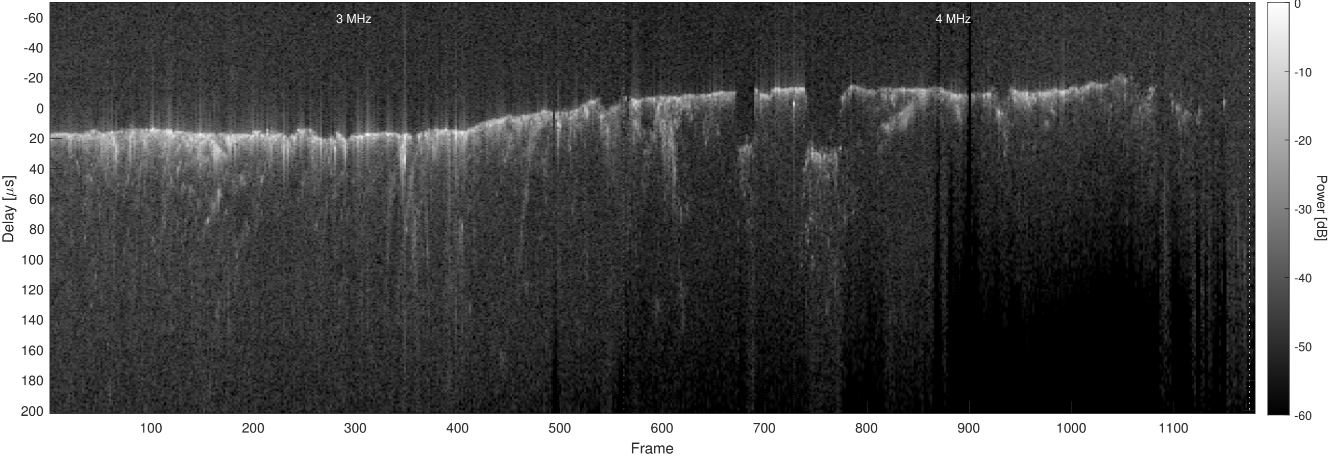
Orbit 9270, Optimized, No Window, Channel 2
