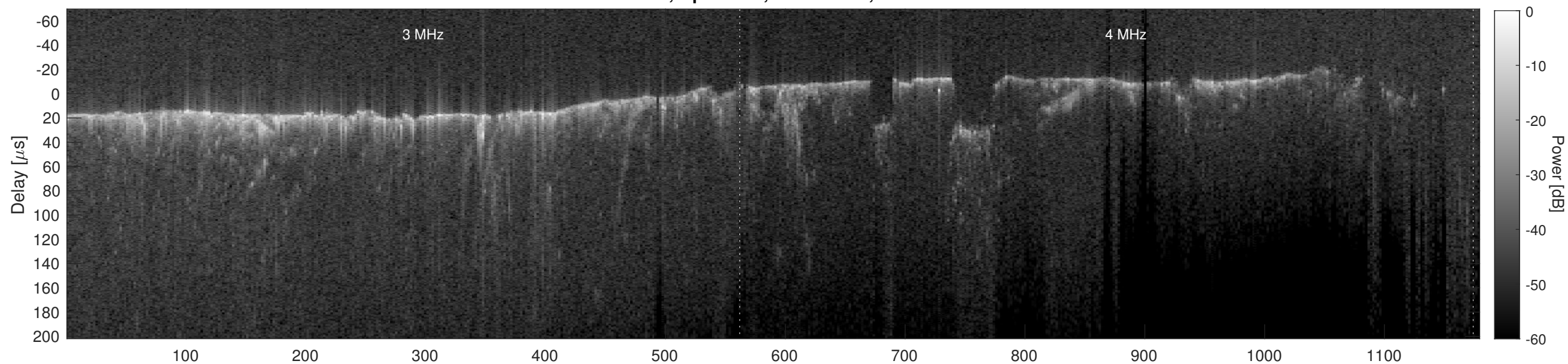
Orbit 9270, Cluttergram
