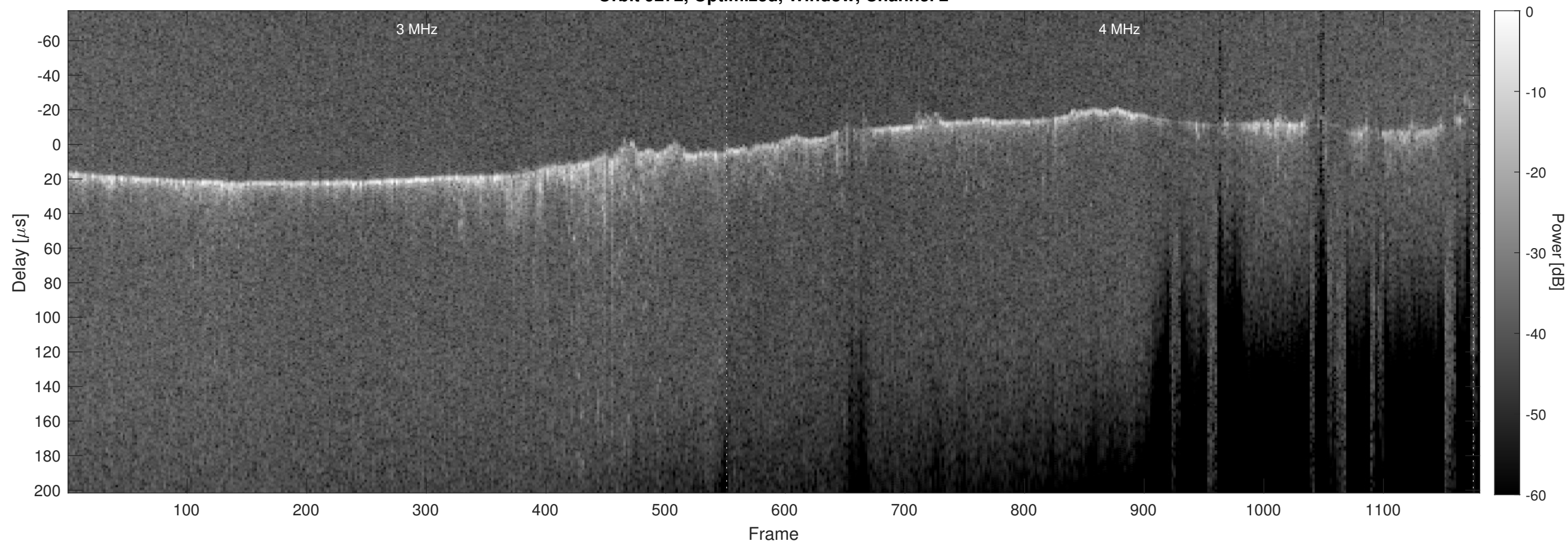
Orbit 9272, Optimized, Window, Channel 2
