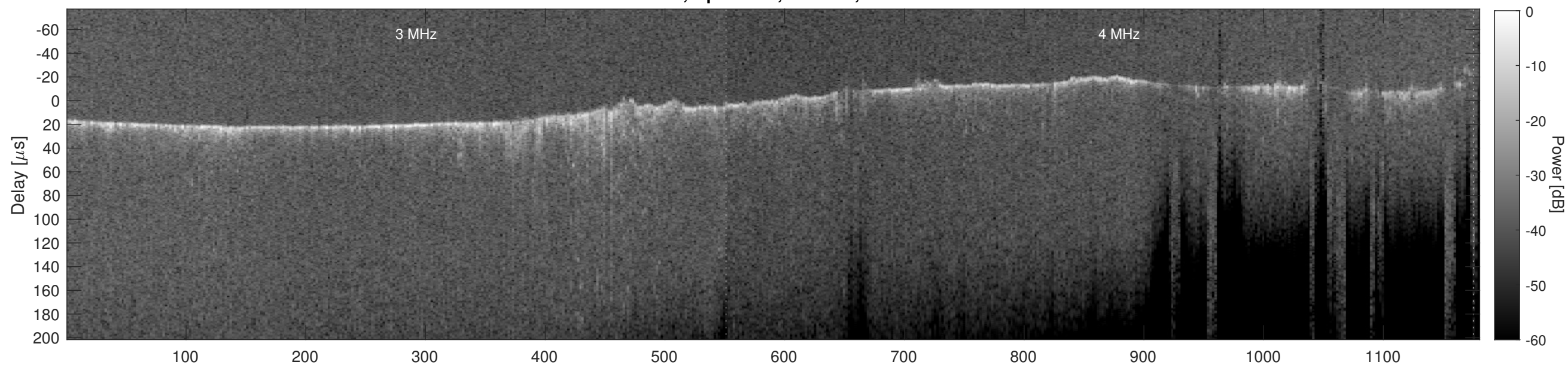
Orbit 9272, Cluttergram
