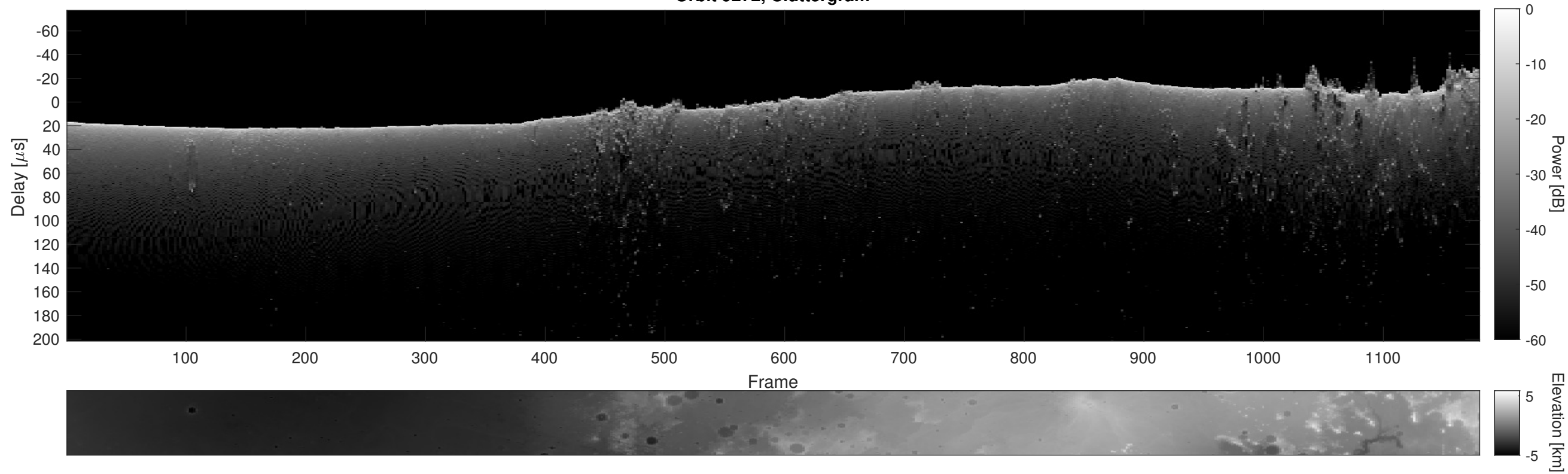
Orbit 9272, Cluttergram
