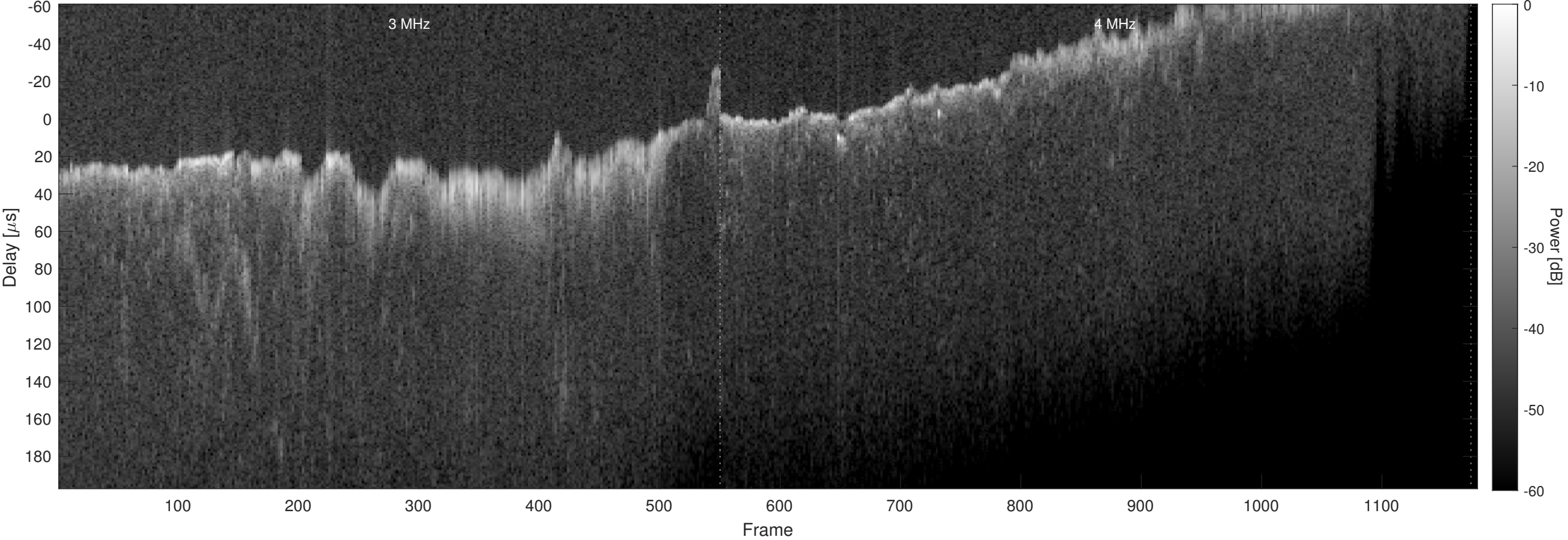
Orbit 9273, Chapman, Window, Channel 2
