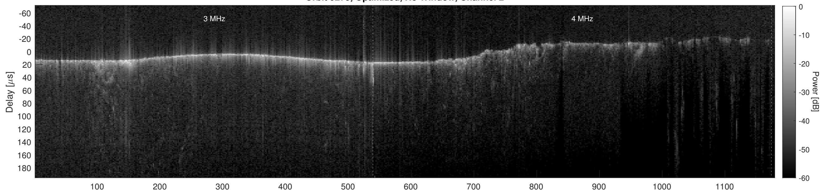
Orbit 9275, Cluttergram
