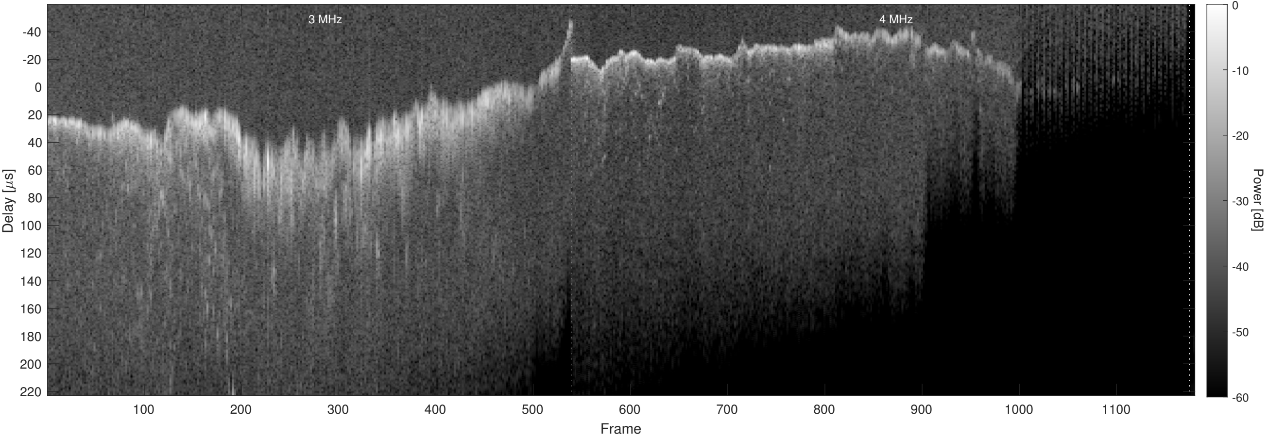
Orbit 9276, Chapman, Window, Channel 2
