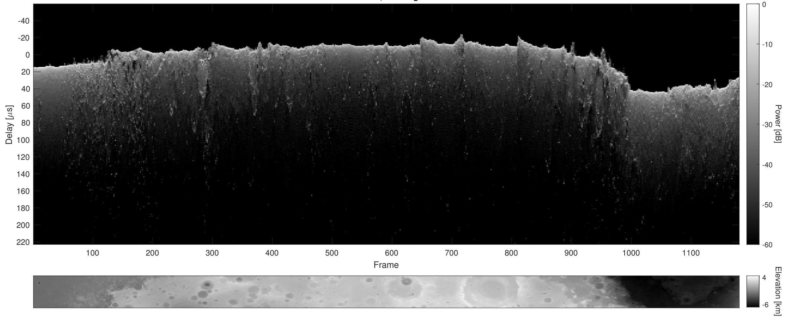
Orbit 9276, Cluttergram
