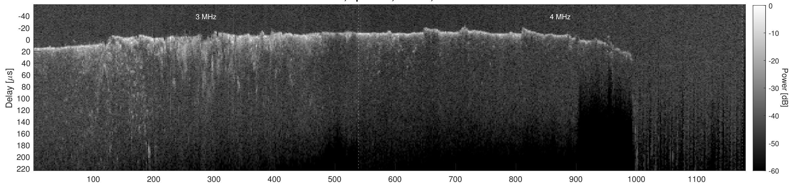
Orbit 9276, Cluttergram
