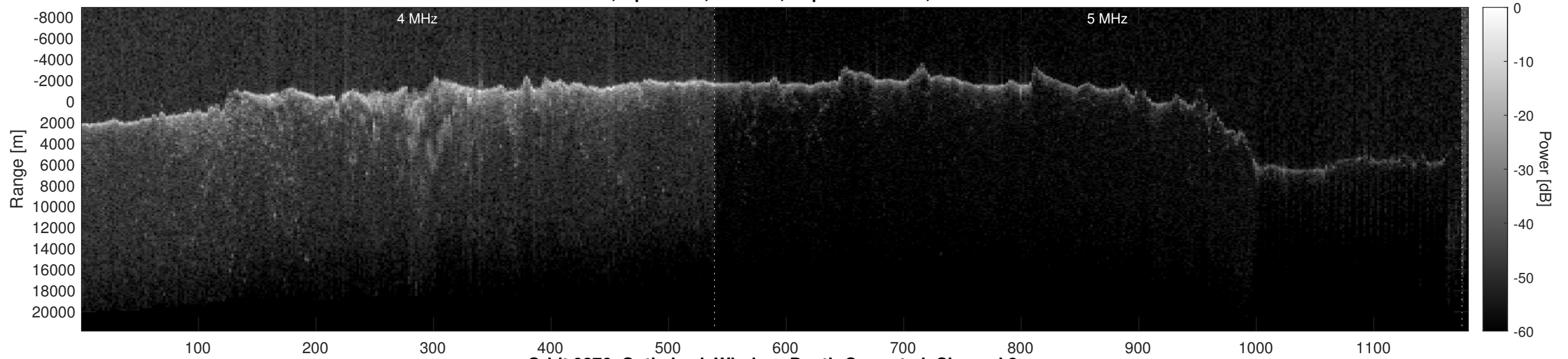
Orbit 9276, Optimized, Window, Depth-Corrected, Channel 2
