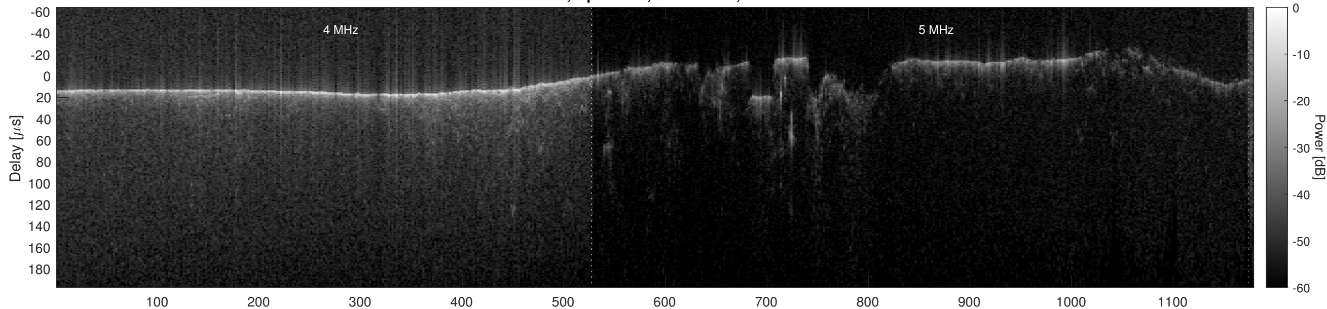
Orbit 9277, Optimized, No Window, Channel 2
