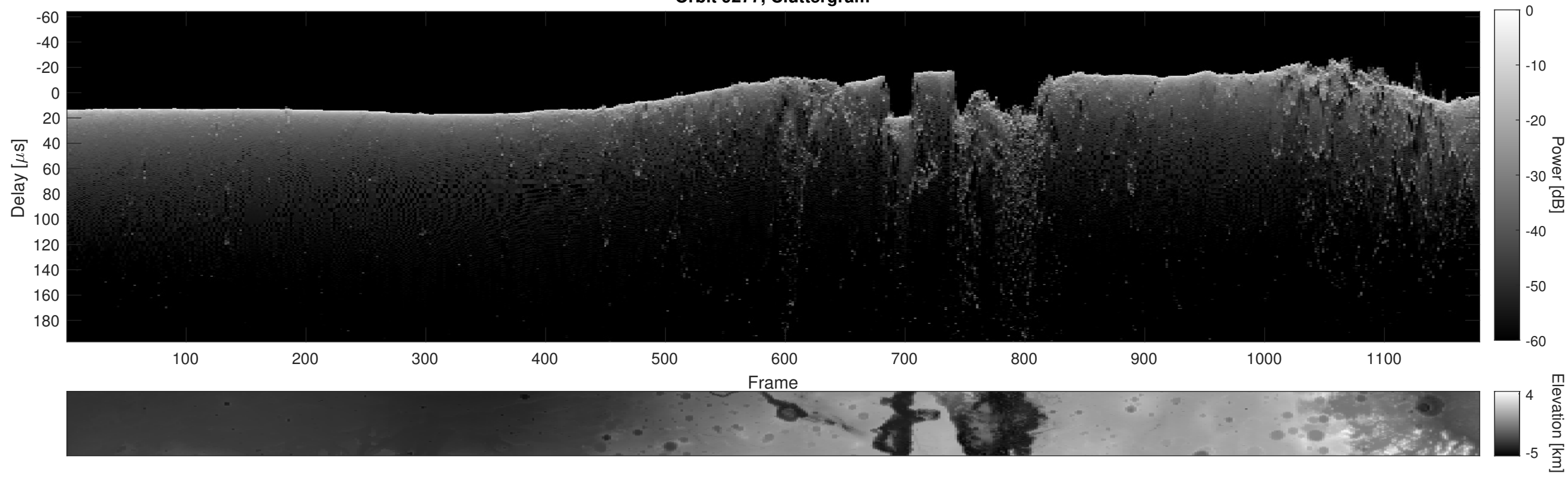
Orbit 9277, Cluttergram
