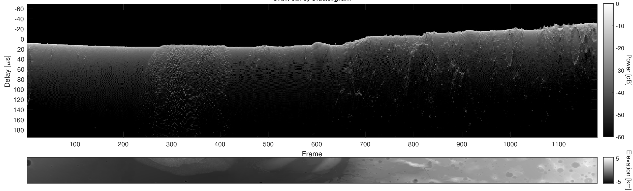
Orbit 9278, Cluttergram
