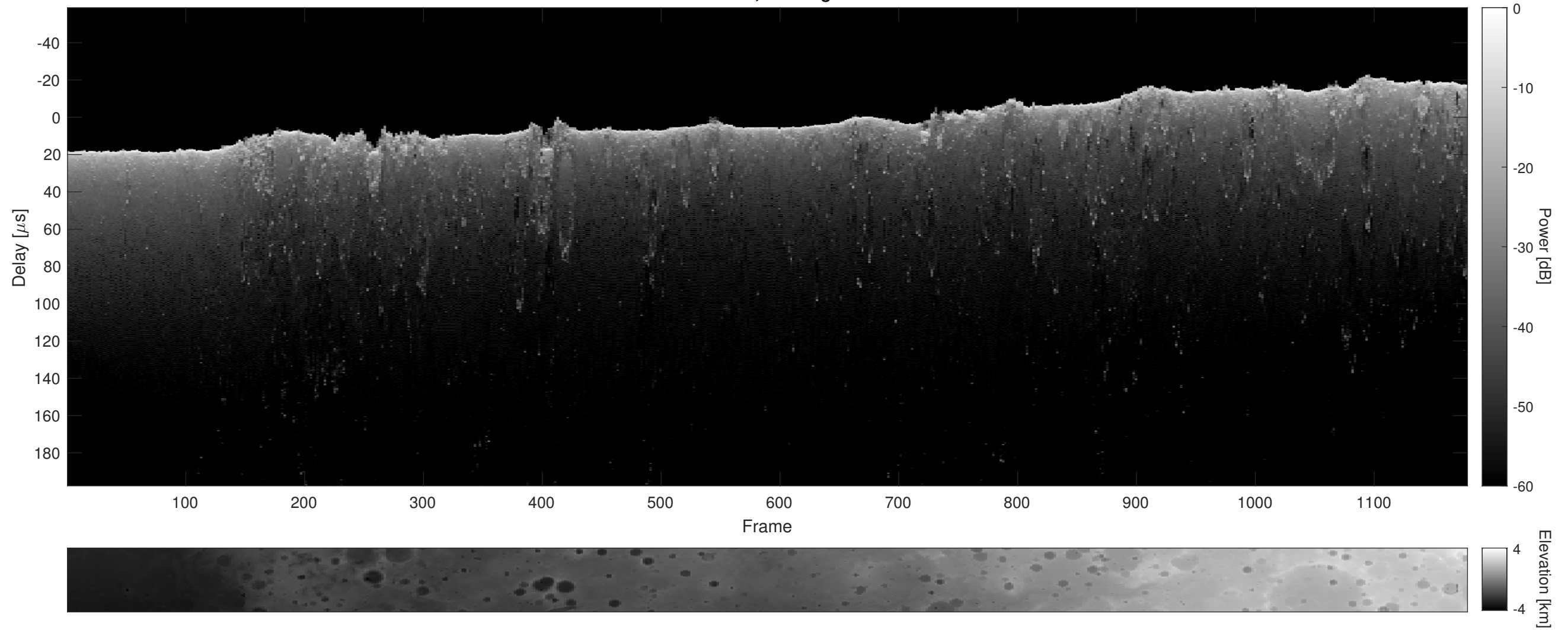
Orbit 9280, Cluttergram
