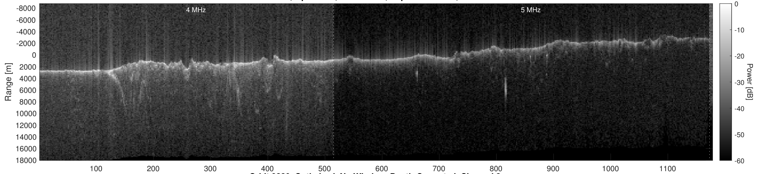
Orbit 9280, Optimized, No Window, Depth-Corrected, Channel 2
