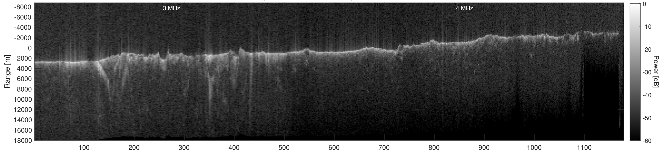
Orbit 9280, Depth-Corrected Cluttergram
