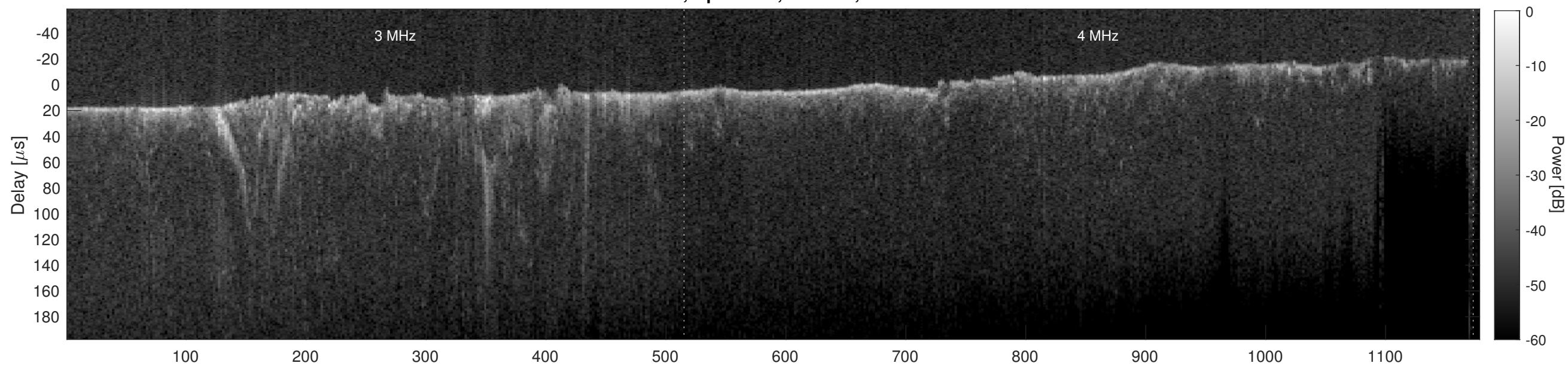
Orbit 9280, Cluttergram
