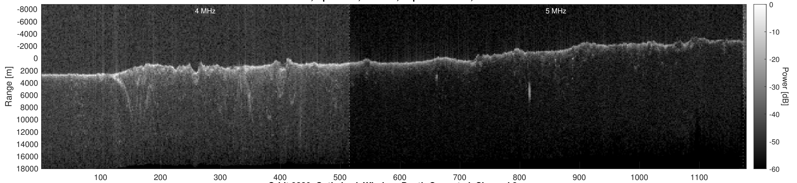
Orbit 9280, Optimized, Window, Depth-Corrected, Channel 2
