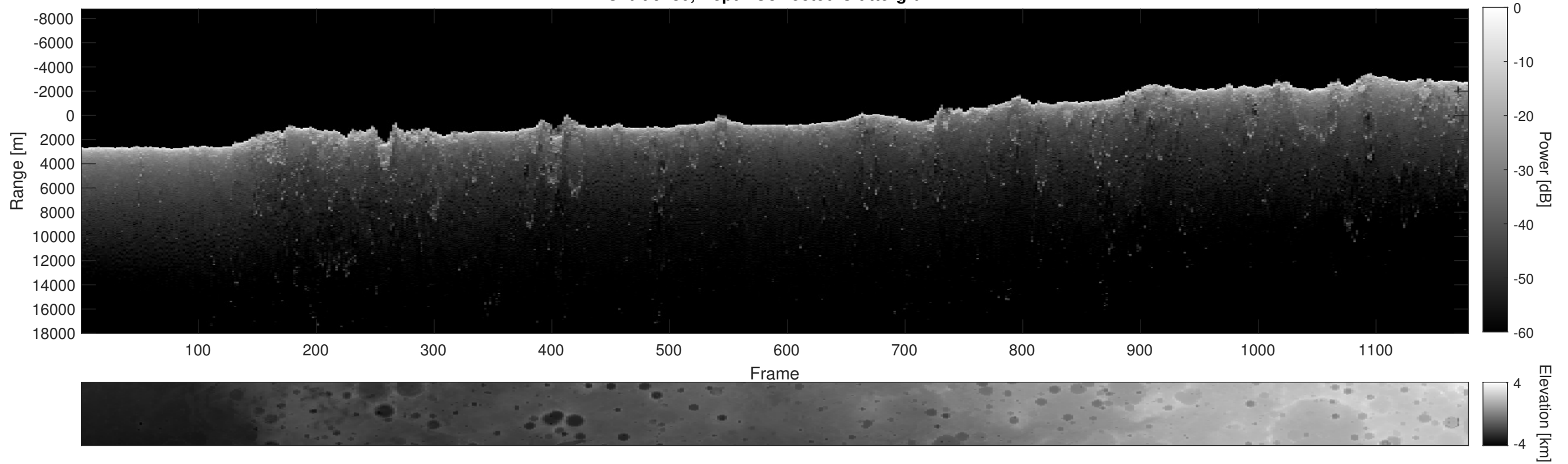
Orbit 9280, Depth-Corrected Cluttergram
