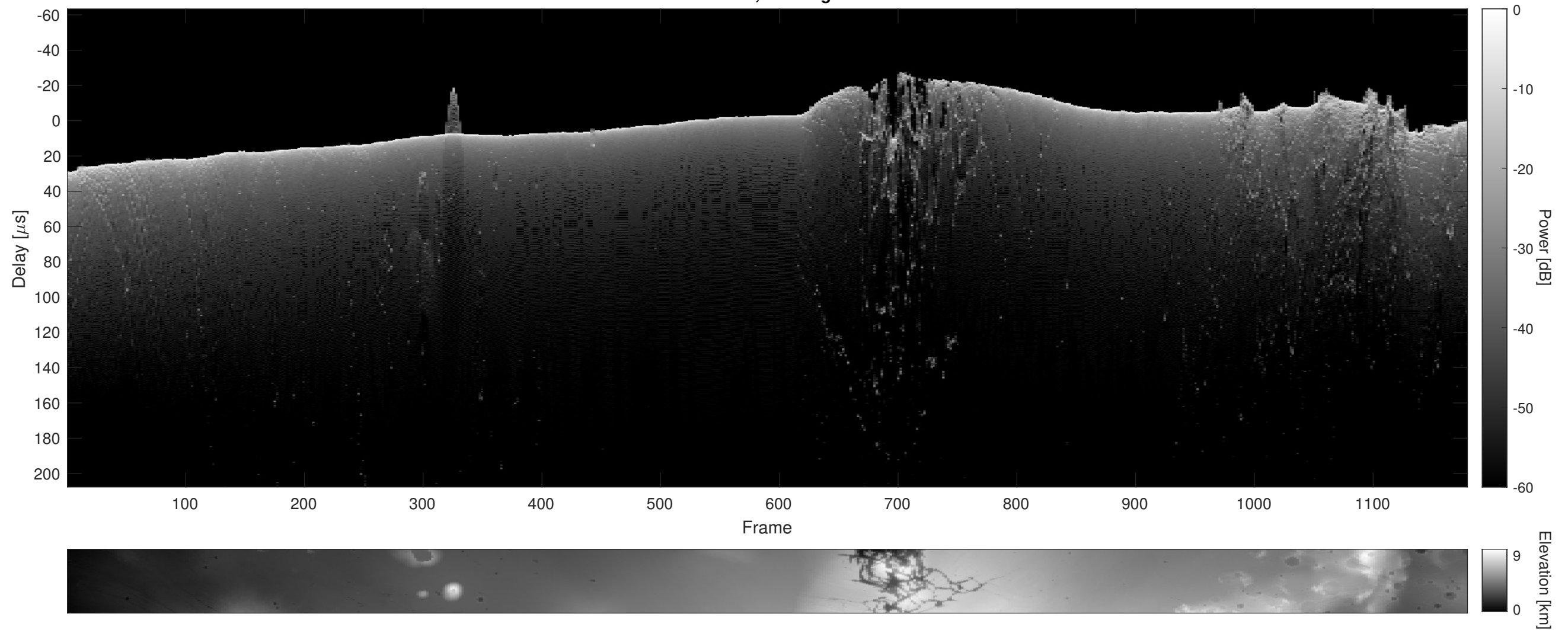
Orbit 9281, Cluttergram
