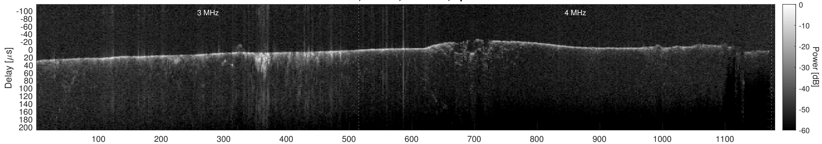
Orbit 9281, Cluttergram
