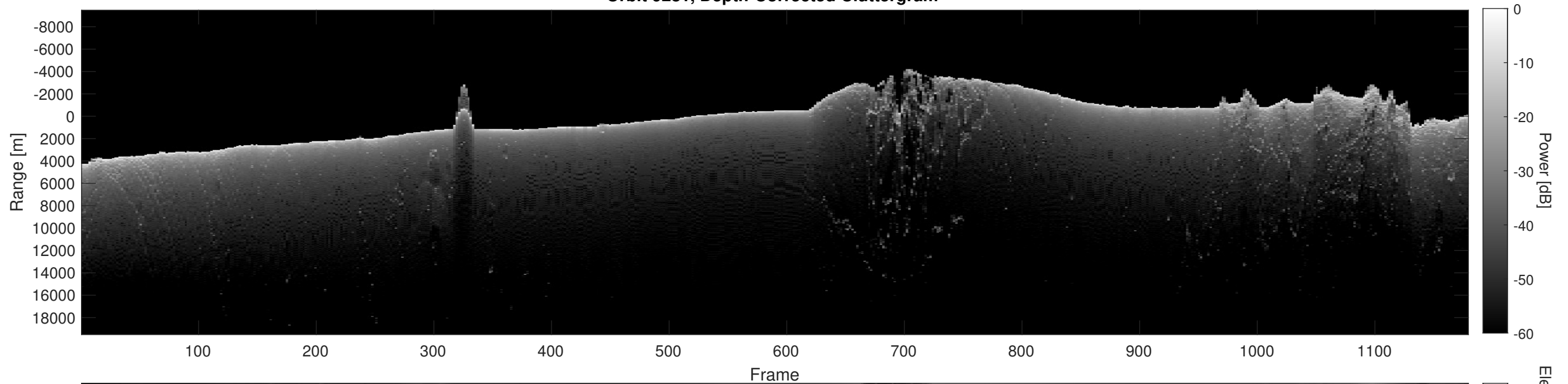
Orbit 9281, Depth-Corrected Cluttergram
