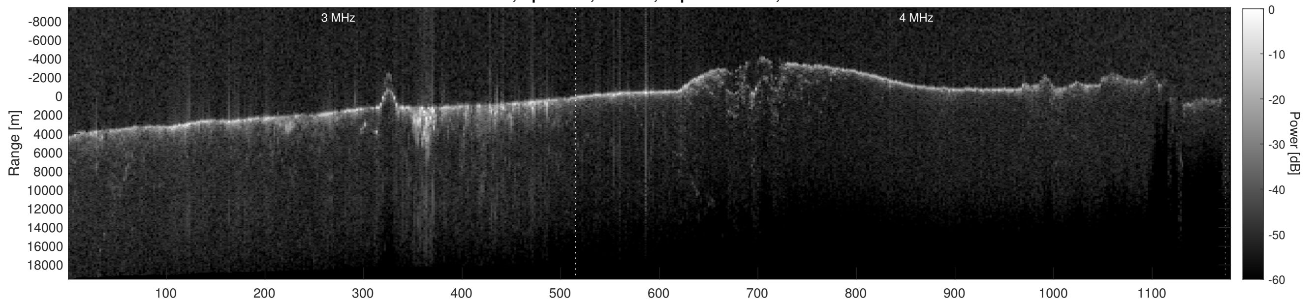
Orbit 9281, Depth-Corrected Cluttergram
