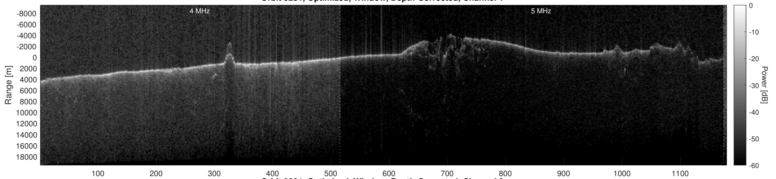
Orbit 9281, Optimized, Window, Depth-Corrected, Channel 2
