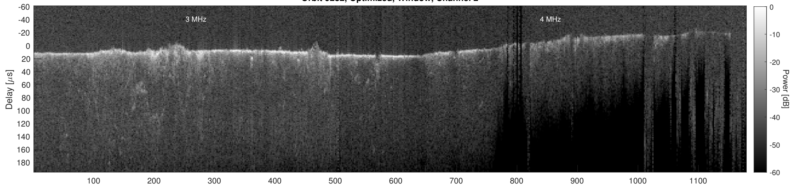
Orbit 9282, Cluttergram
