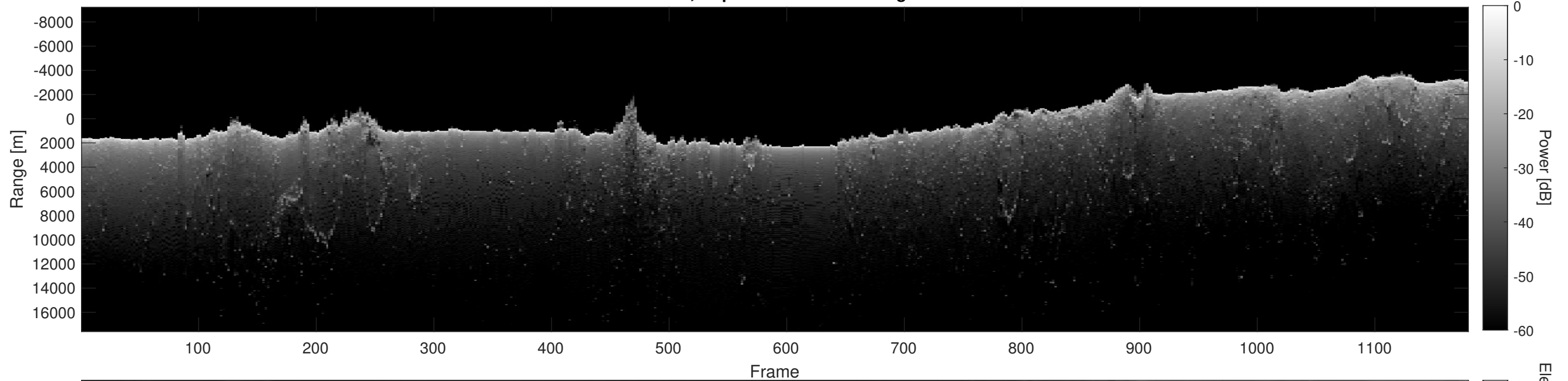
Orbit 9282, Depth-Corrected Cluttergram
