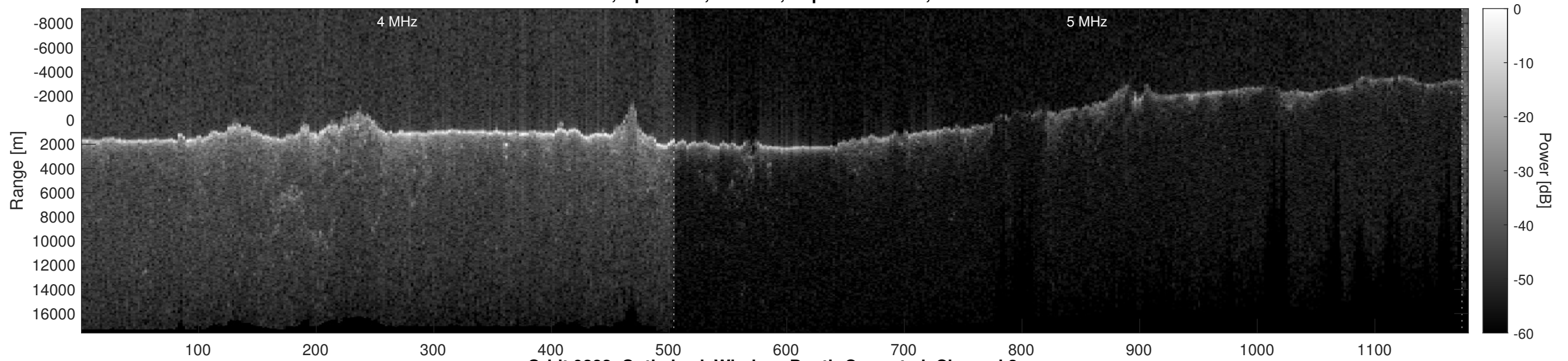
Orbit 9282, Optimized, Window, Depth-Corrected, Channel 2
