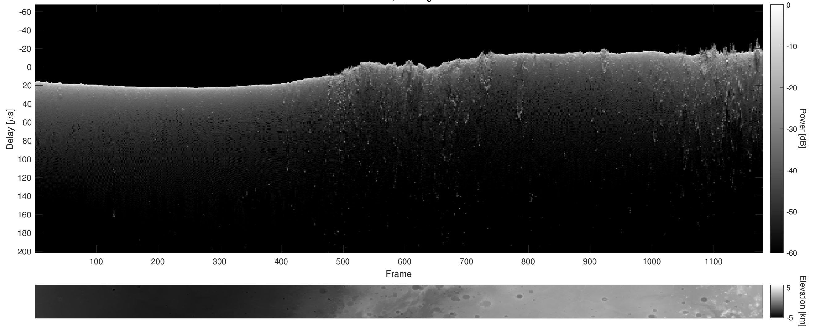
Orbit 9286, Cluttergram
