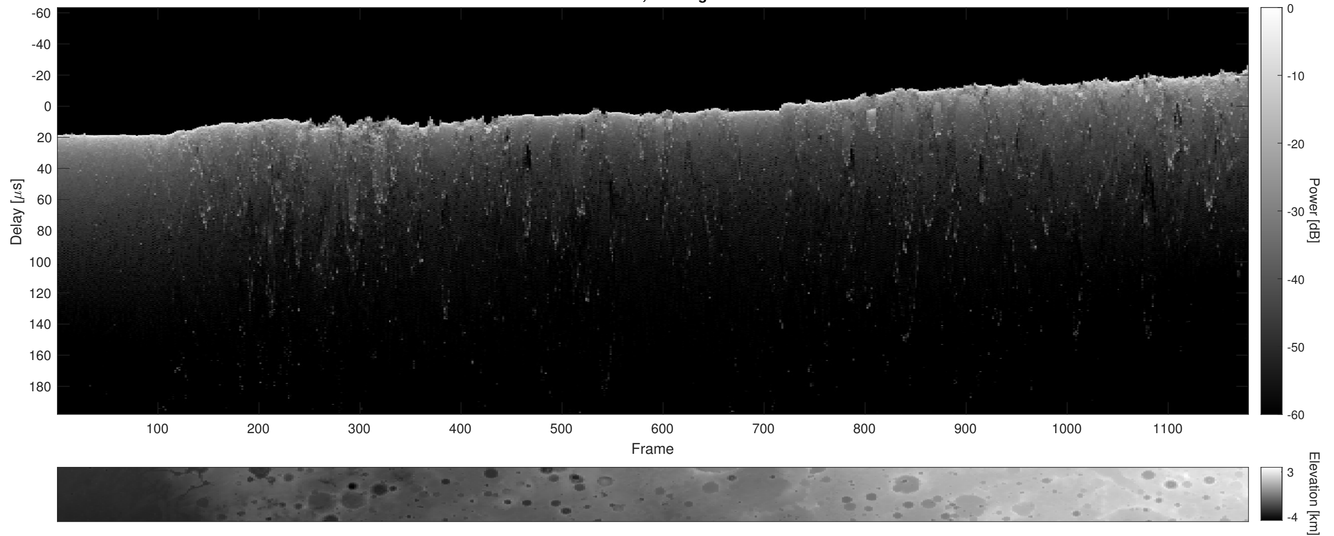
Orbit 9287, Cluttergram
