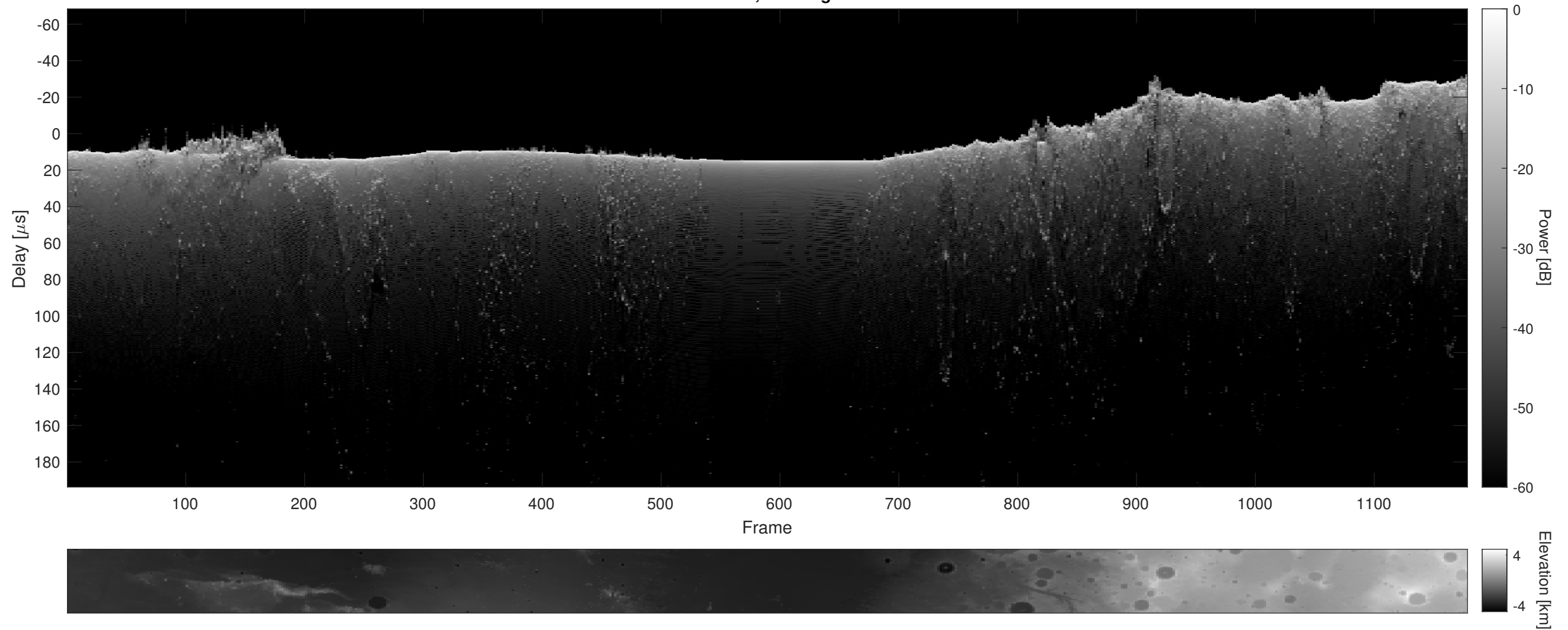
Orbit 9289, Cluttergram
