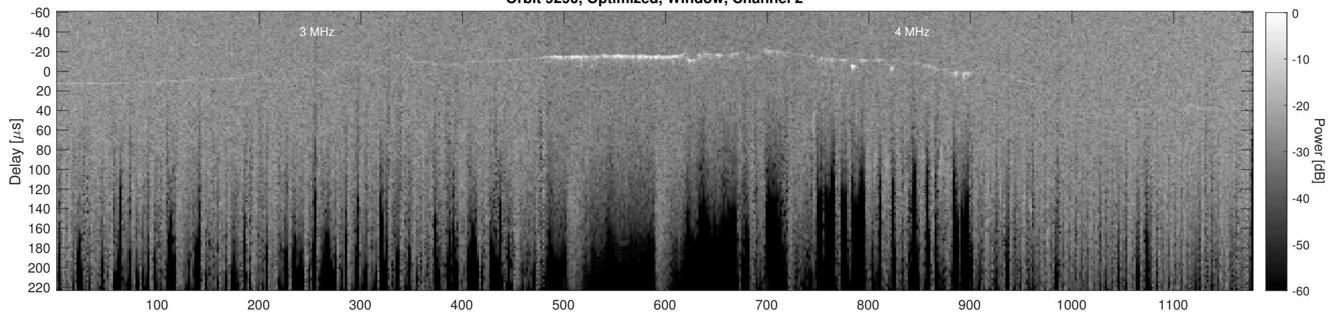
Orbit 9290, Cluttergram
