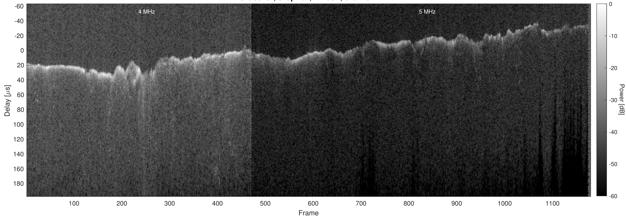
Orbit 9292, Chapman, Window, Channel 2
