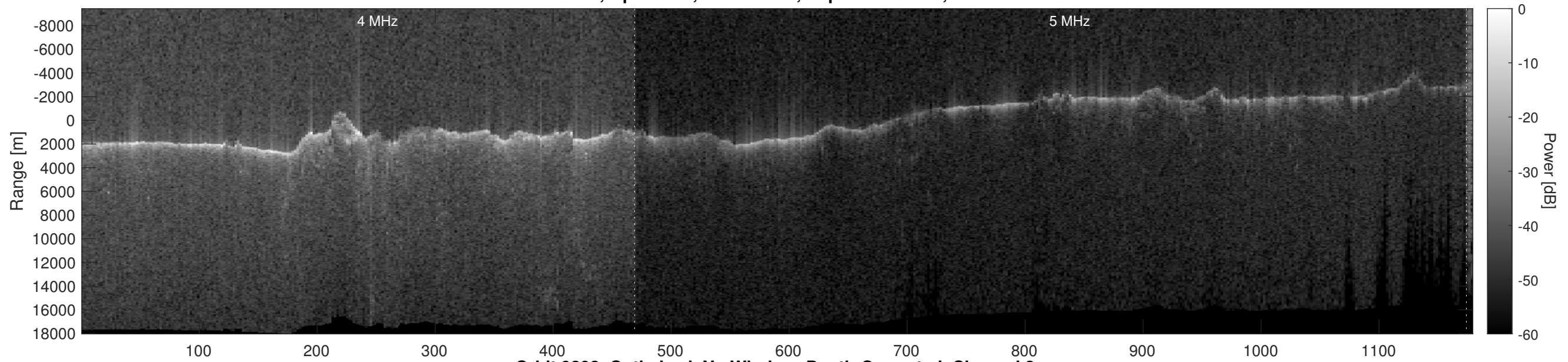
Orbit 9292, Optimized, No Window, Depth-Corrected, Channel 2
