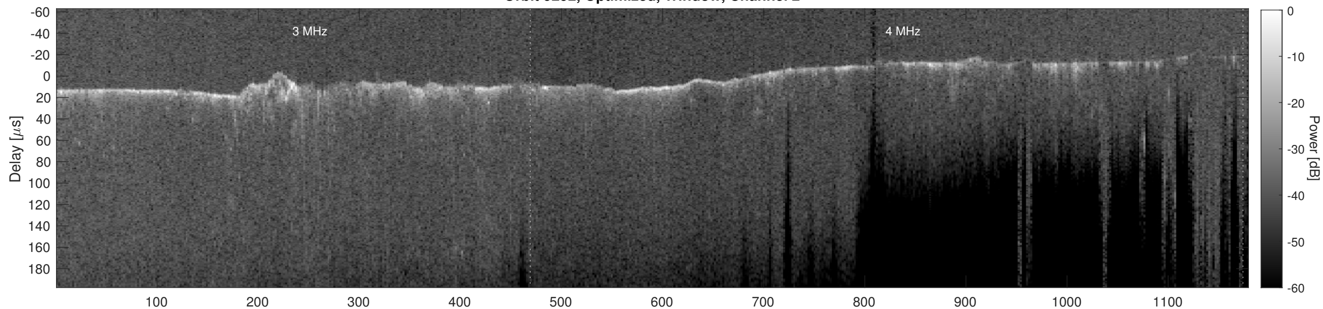
Orbit 9292, Cluttergram
