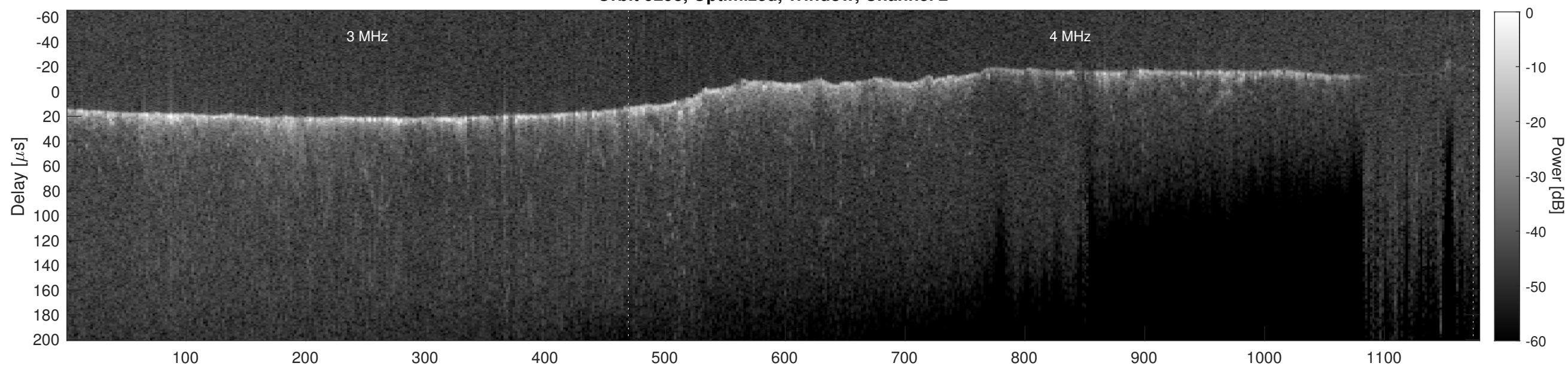
Orbit 9293, Cluttergram
