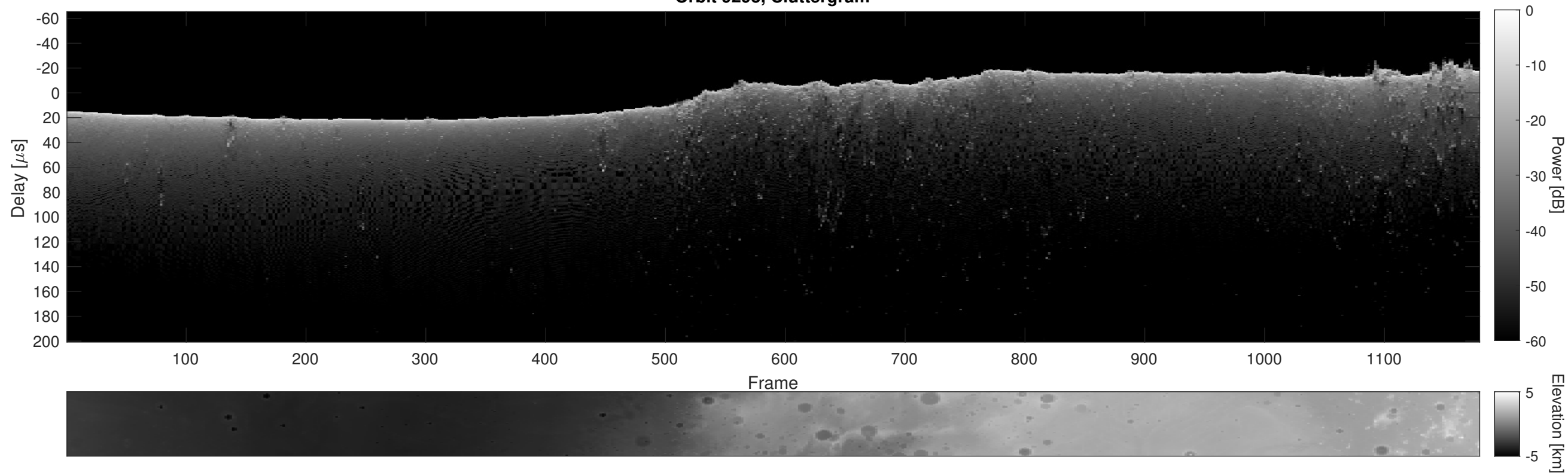
Orbit 9293, Cluttergram
