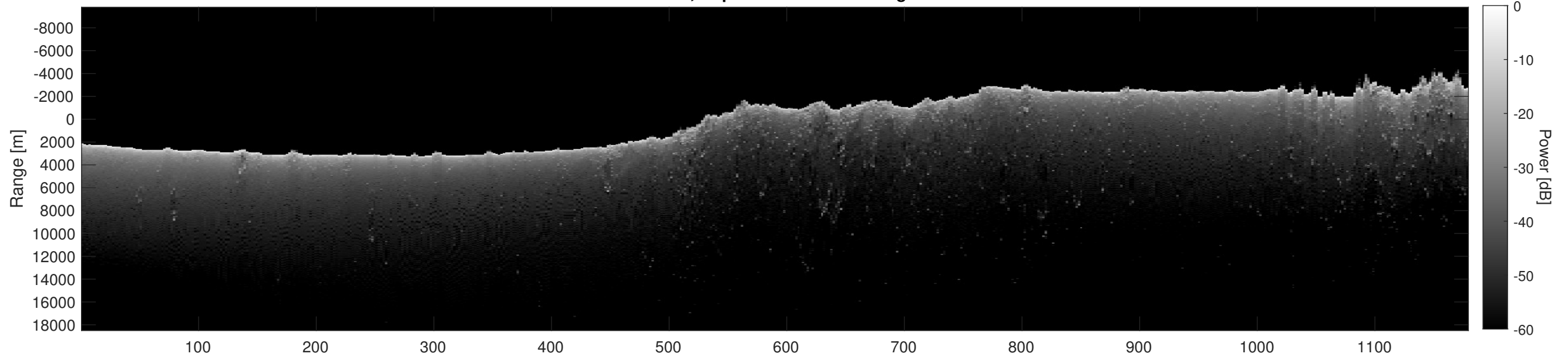
Orbit 9293, Depth-Corrected Cluttergram
