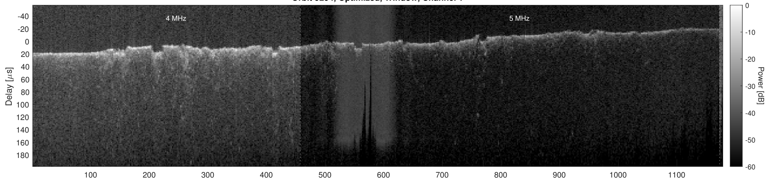
Orbit 9294, Optimized, Window, Channel 2
