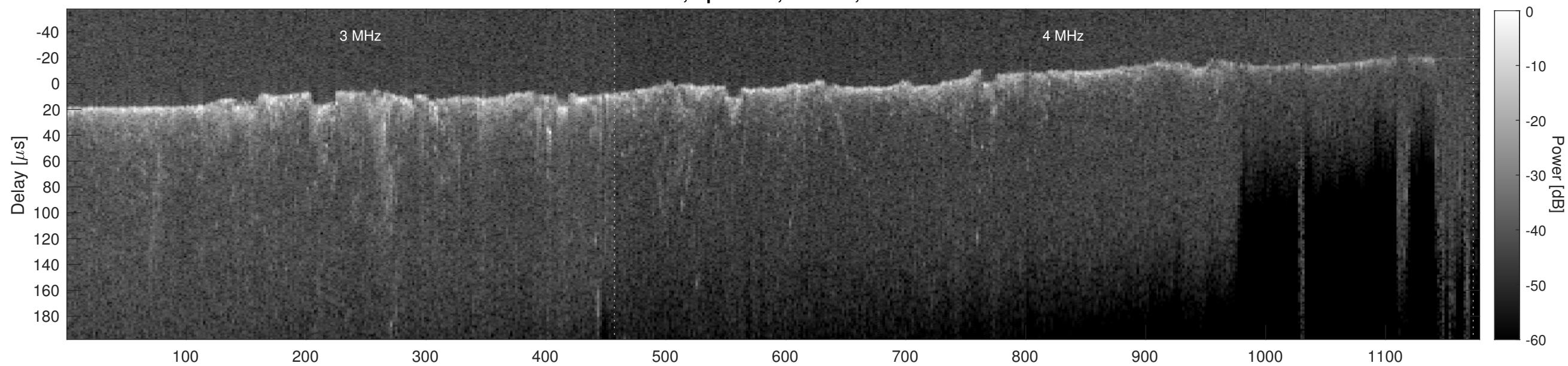
Orbit 9294, Cluttergram
