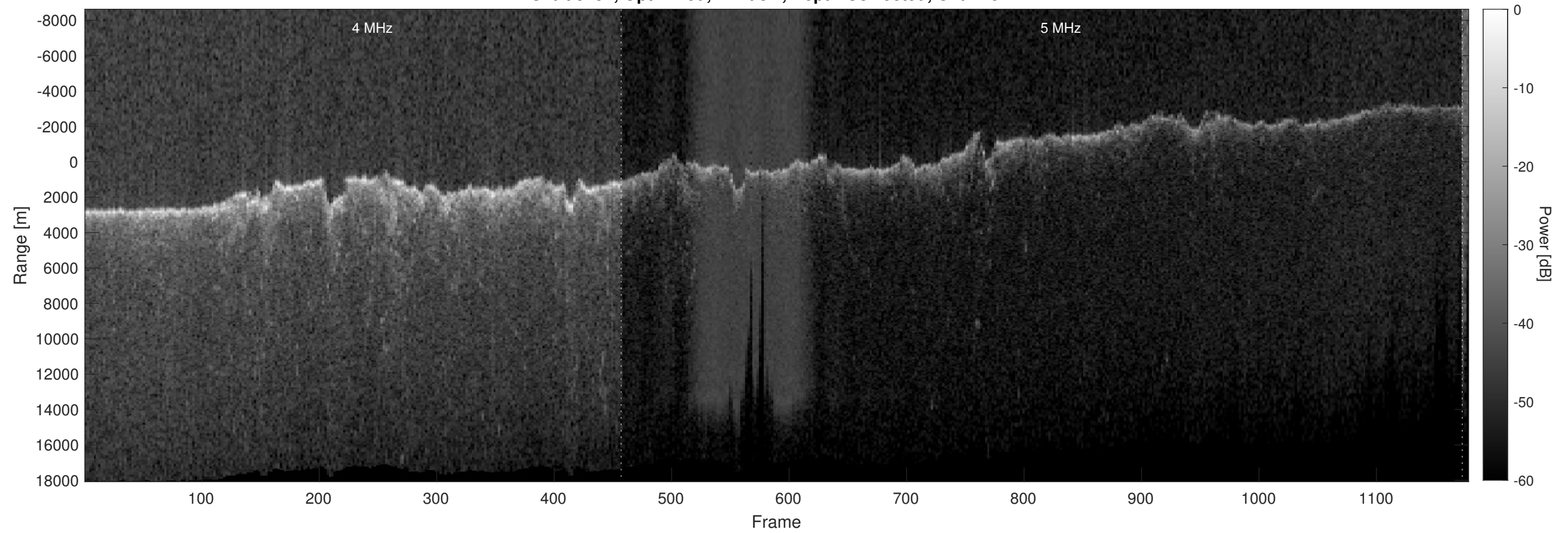
Orbit 9294, Optimized, Window, Depth-Corrected, Channel 2
