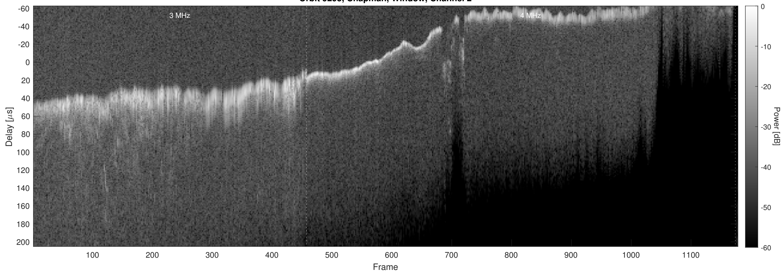
Orbit 9295, Chapman, Window, Channel 2
