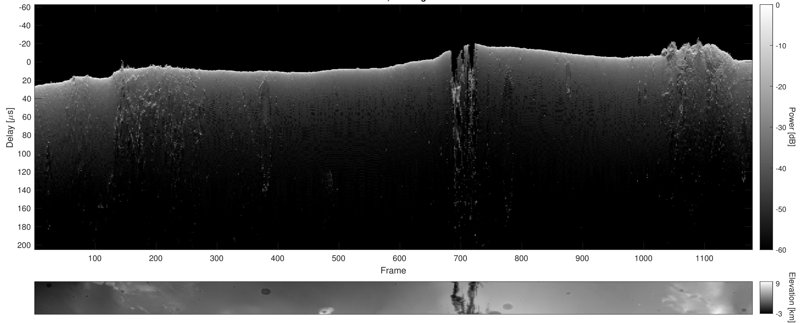
Orbit 9295, Cluttergram
