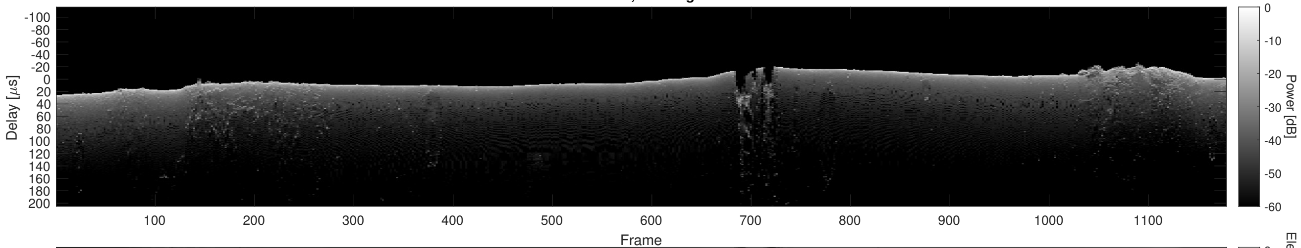
Orbit 9295, Cluttergram
