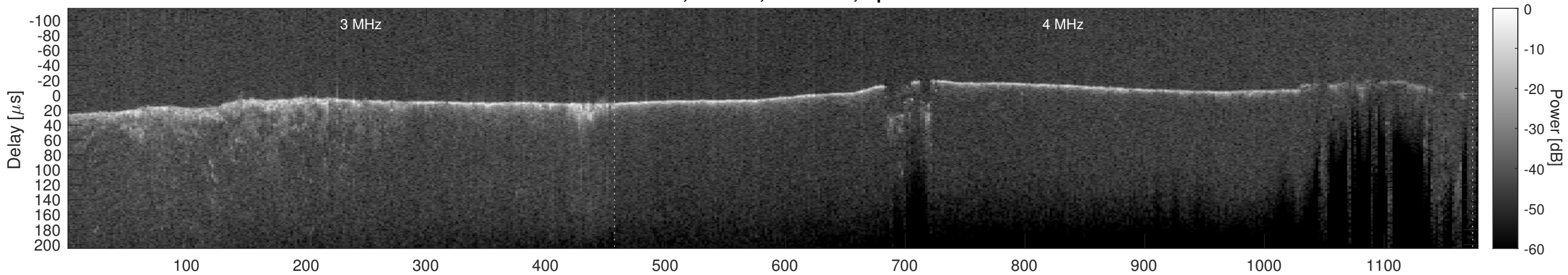
Orbit 9295, Cluttergram
