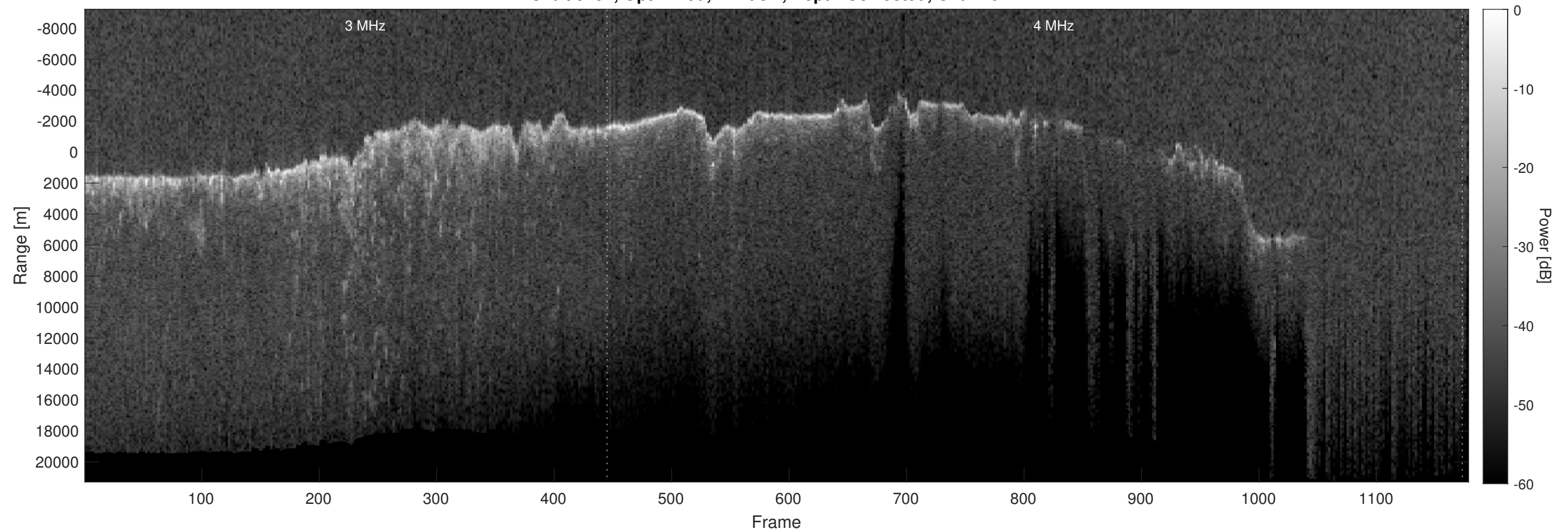
Orbit 9297, Optimized, Window, Depth-Corrected, Channel 2
