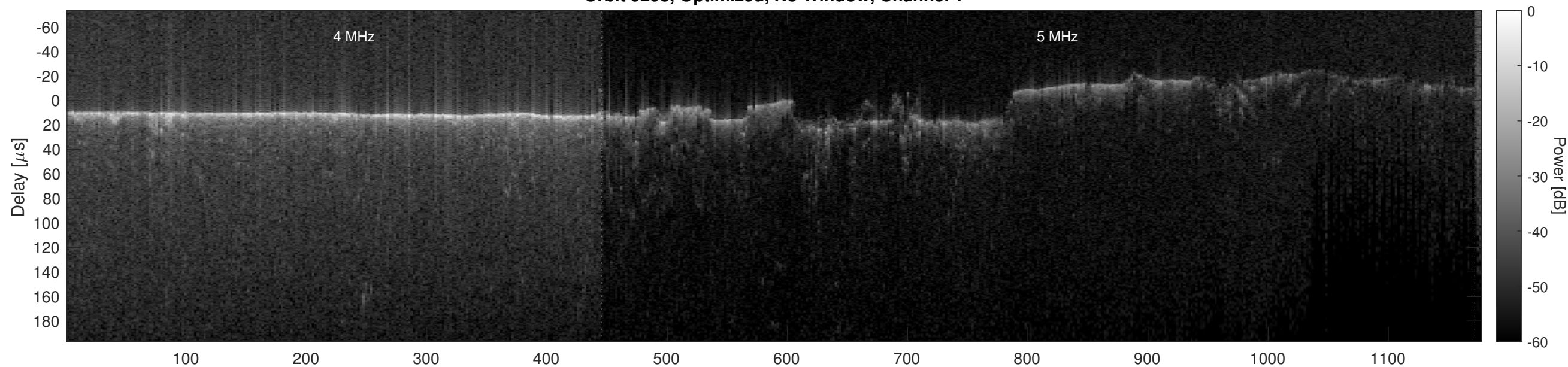
Orbit 9298, Optimized, No Window, Channel 2
