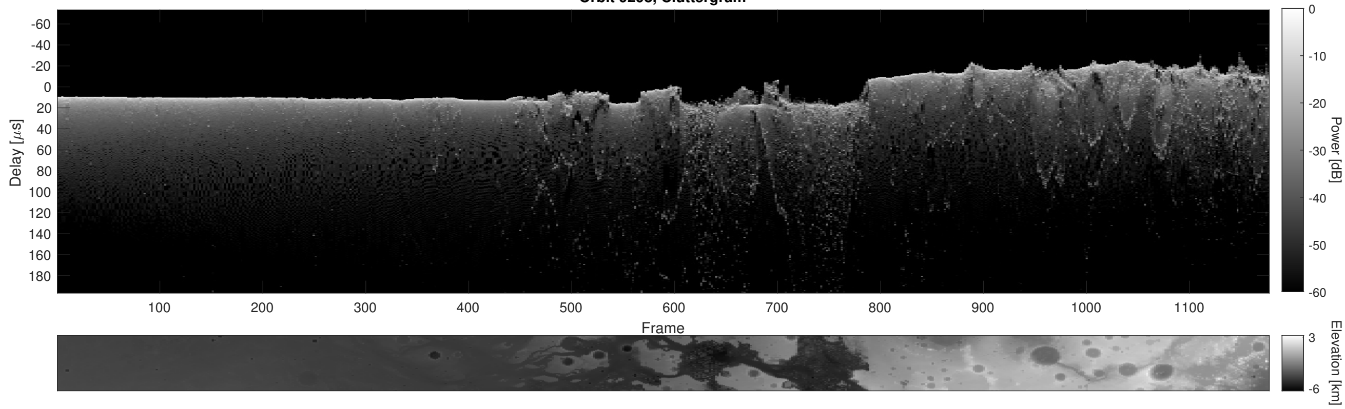
Orbit 9298, Cluttergram
