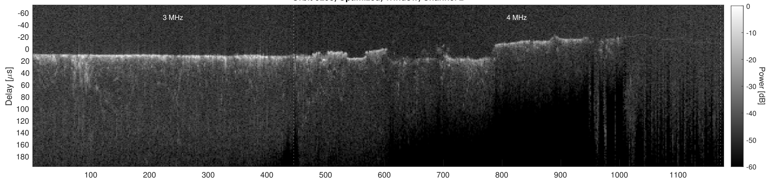
Orbit 9298, Cluttergram
