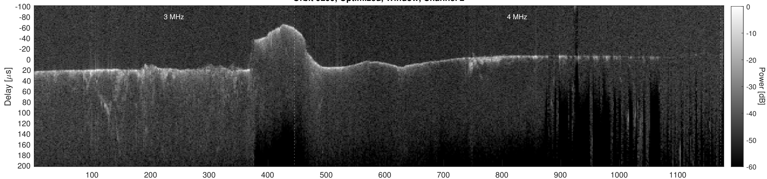
Orbit 9299, Cluttergram
