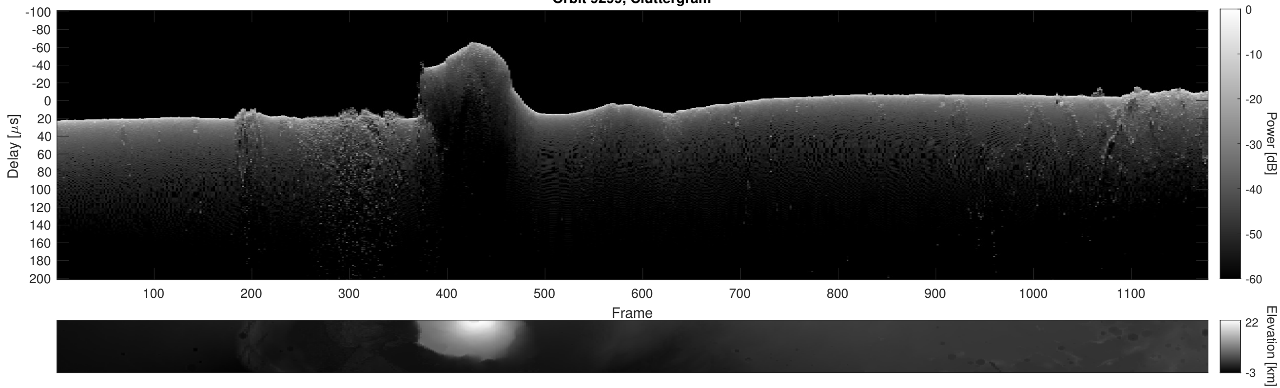
Orbit 9299, Cluttergram
