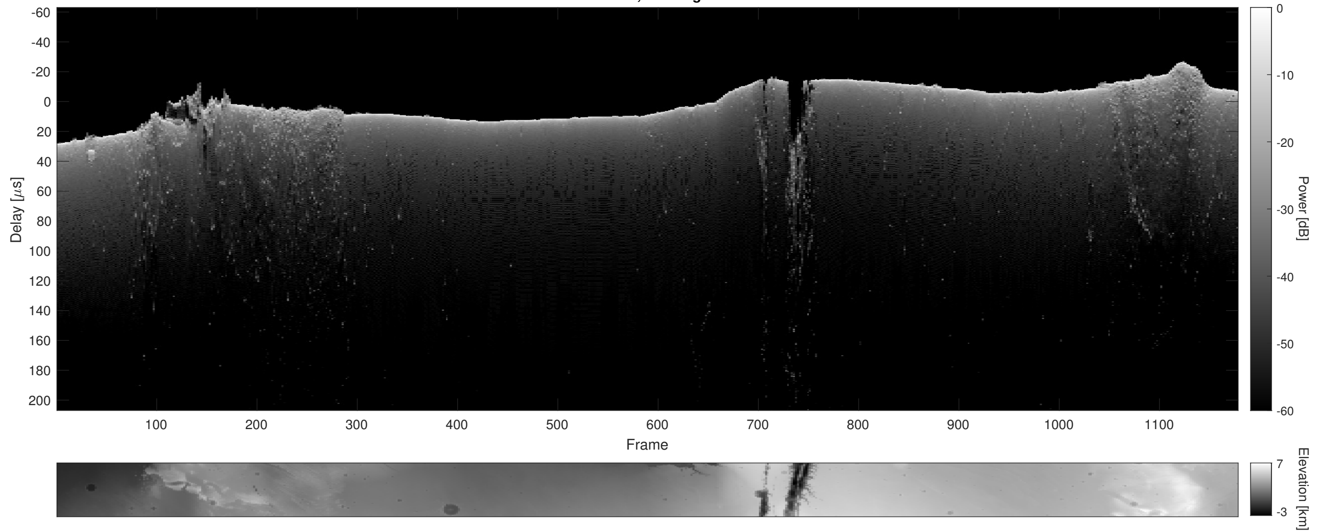
Orbit 9302, Cluttergram
