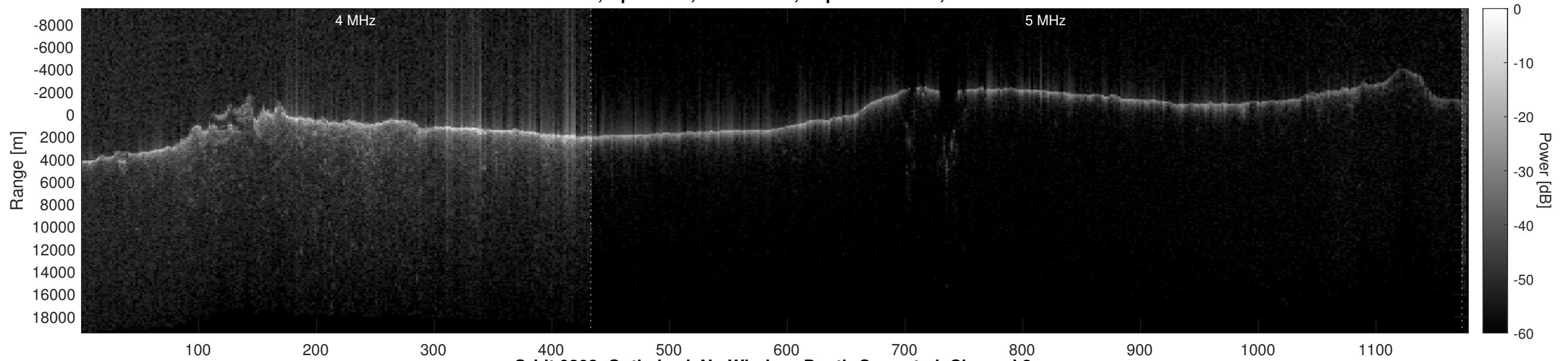
Orbit 9302, Optimized, No Window, Depth-Corrected, Channel 2
