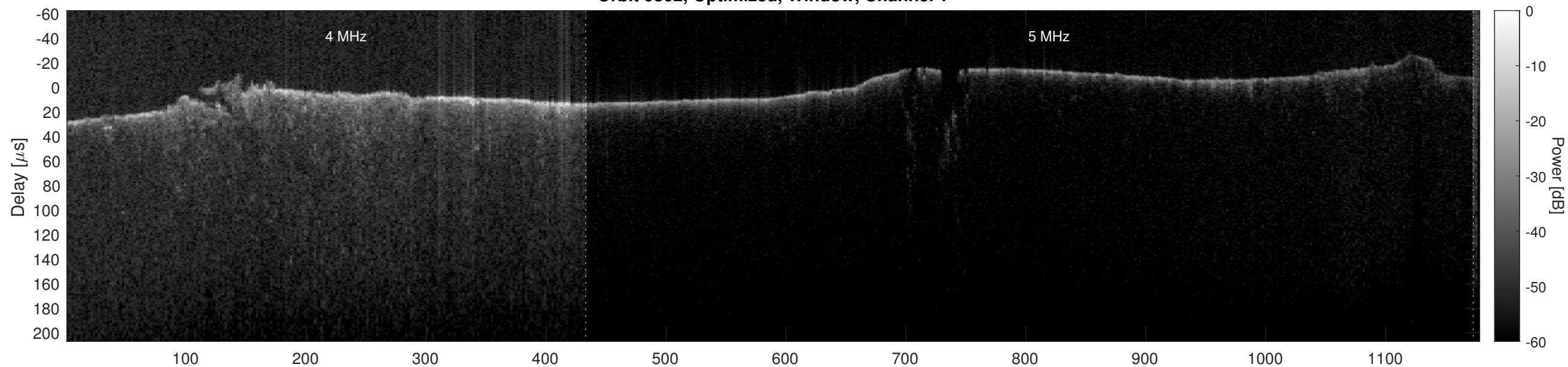
Orbit 9302, Optimized, Window, Channel 2
