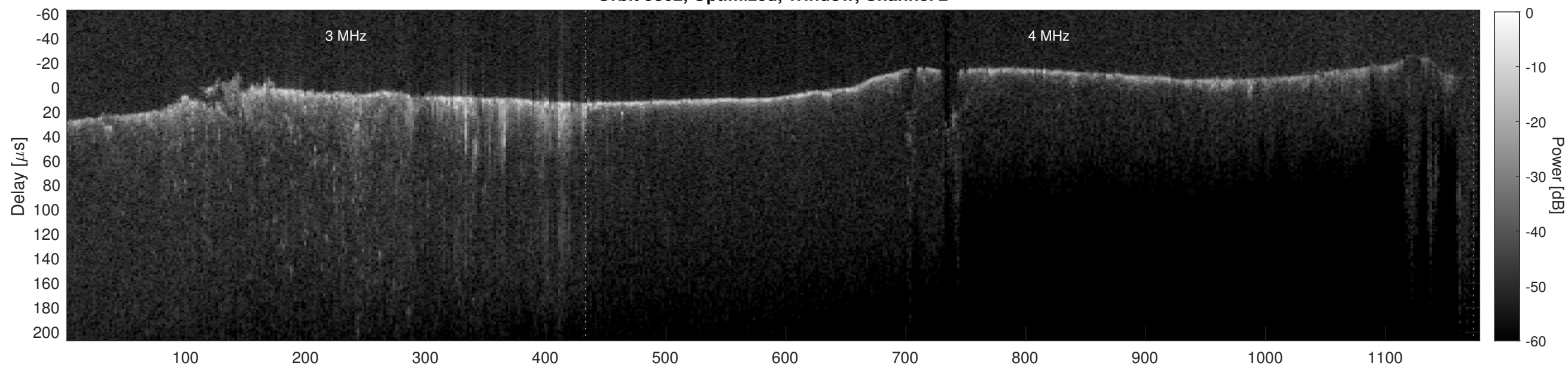
Orbit 9302, Cluttergram
