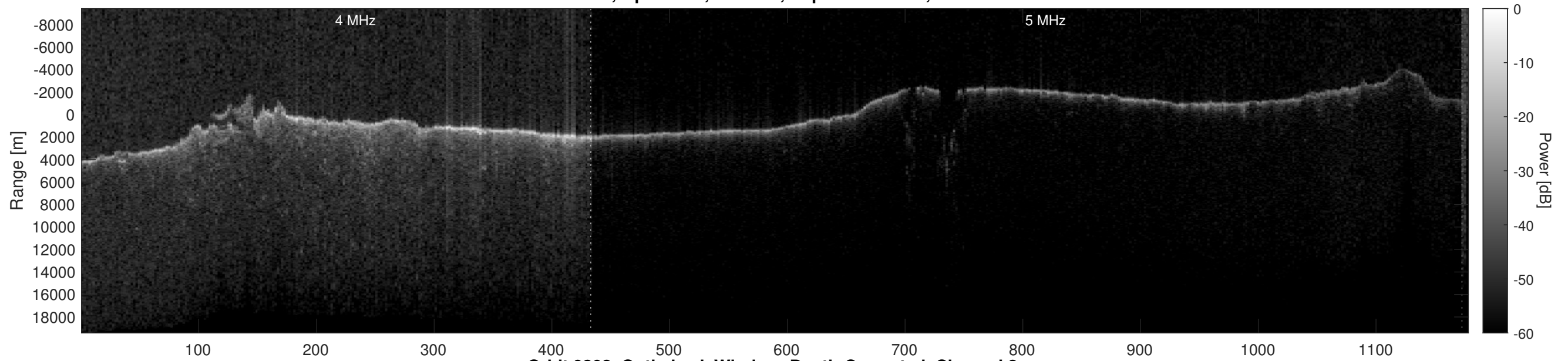
Orbit 9302, Optimized, Window, Depth-Corrected, Channel 2
