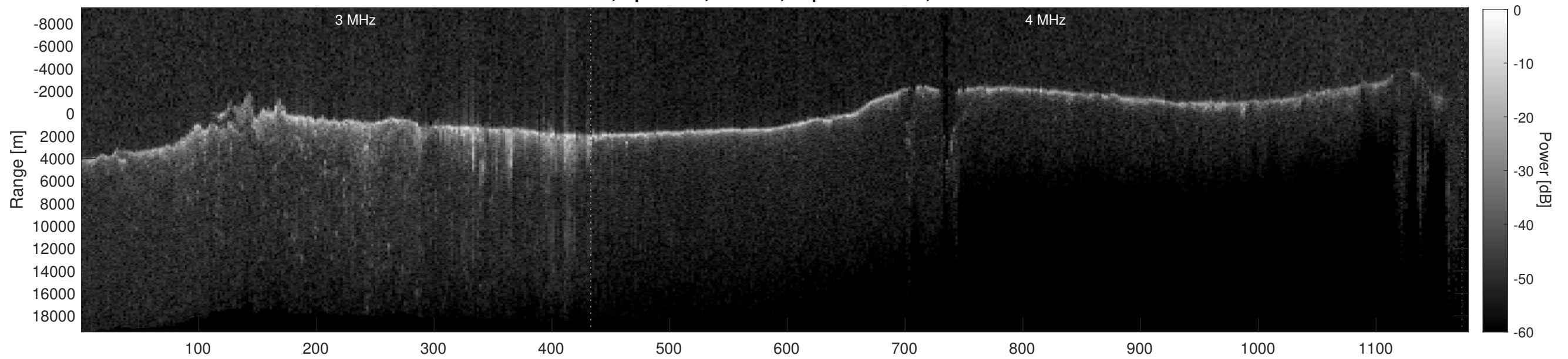
Orbit 9302, Depth-Corrected Cluttergram
