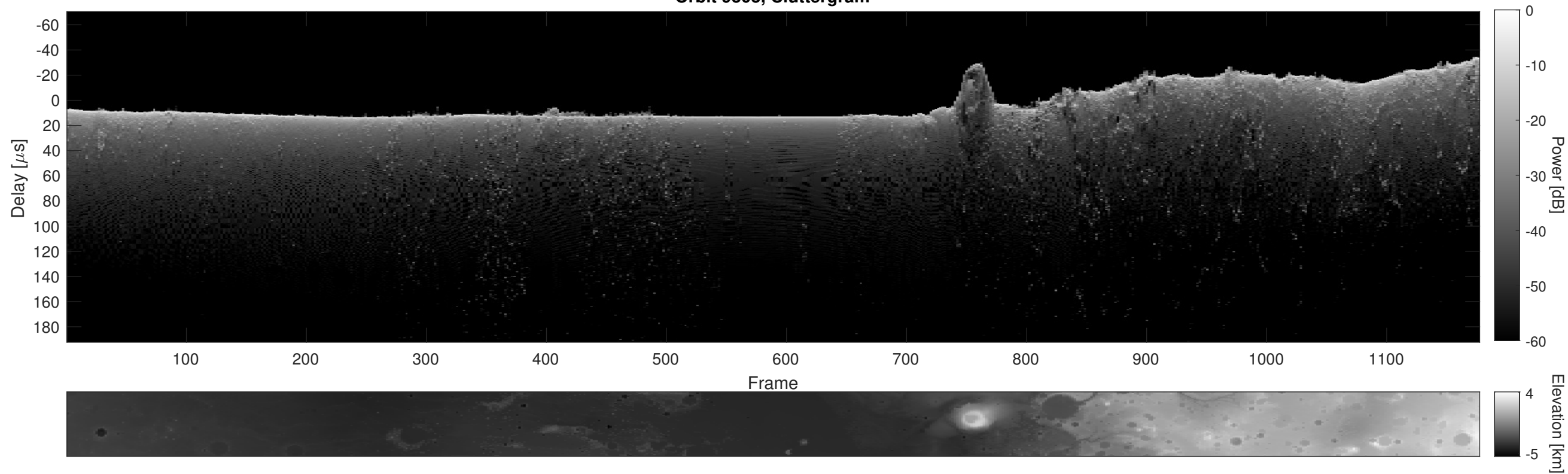
Orbit 9303, Cluttergram
