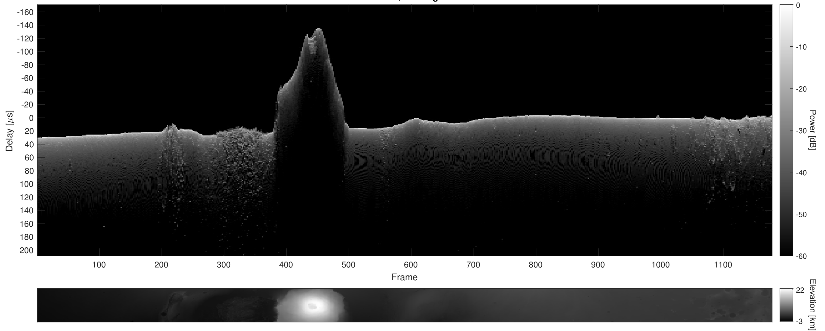
Orbit 9306, Cluttergram
