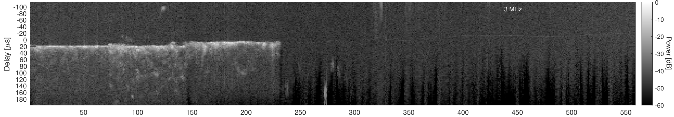
Orbit 9308, Cluttergram
