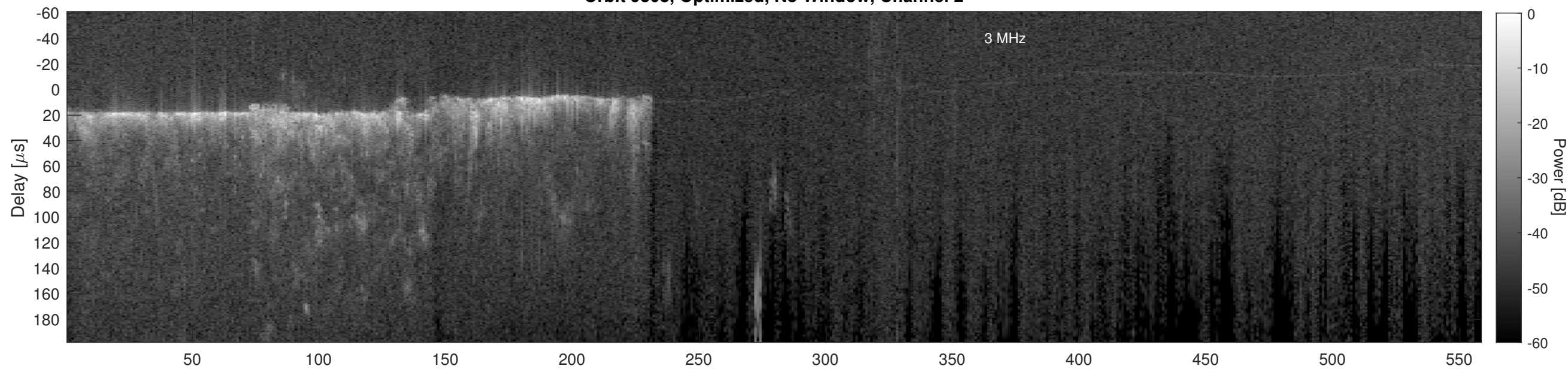
Orbit 9308, Cluttergram
