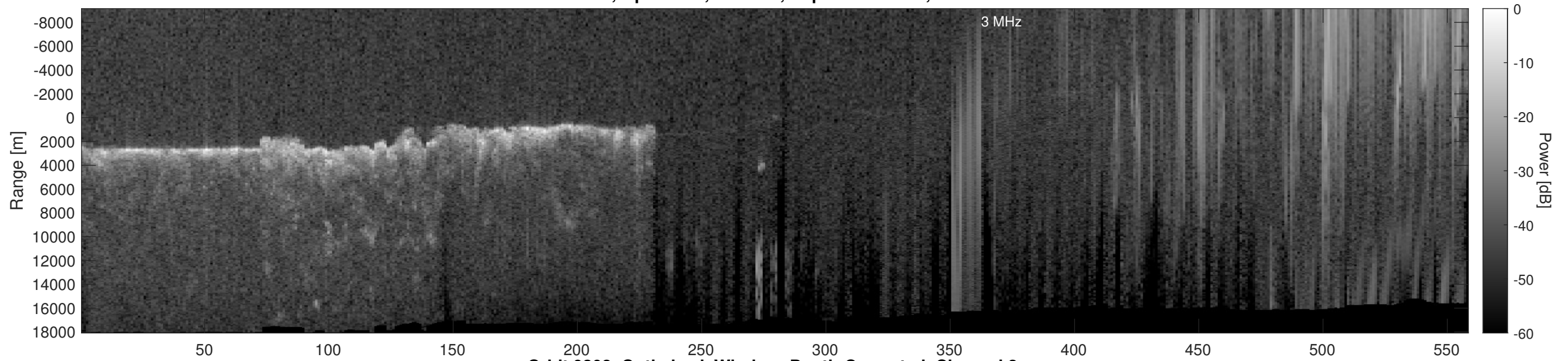
Orbit 9308, Optimized, Window, Depth-Corrected, Channel 2
